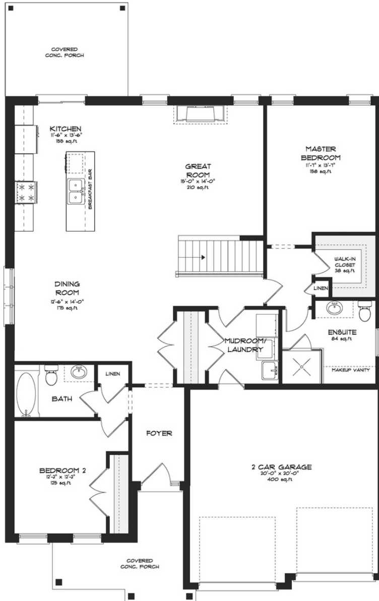
MAIN FLOOR PLAN INTERIOR AREA 1939 sq.ft.
