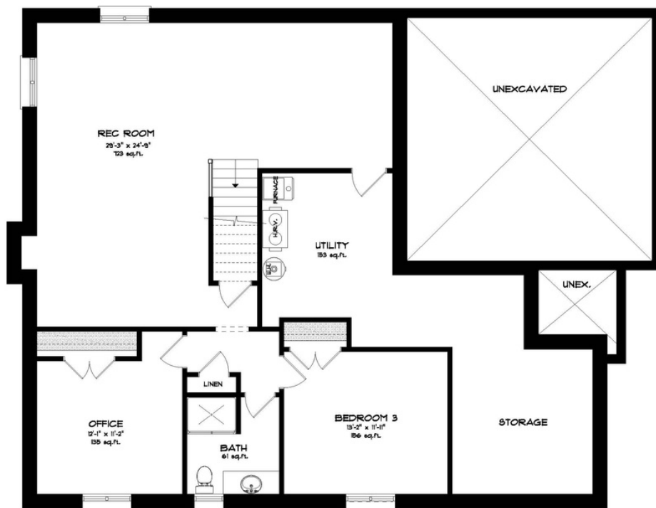
BASEMENT PLAN INTERIOR AREA 908 sq.ft.
